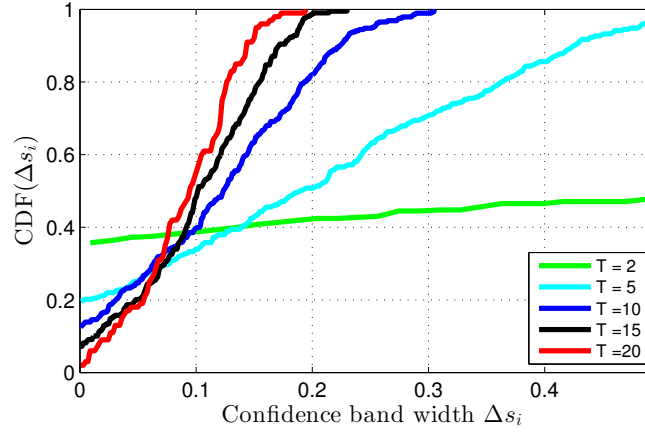
Figure 5: Empirical cumulative distribution function CDF(\Delta s_i) of confidence band widths \Delta s_i(T) after T = 2 (green), 5 (cyan), 10 (blue), 15 (black) and 20 (red) days.
