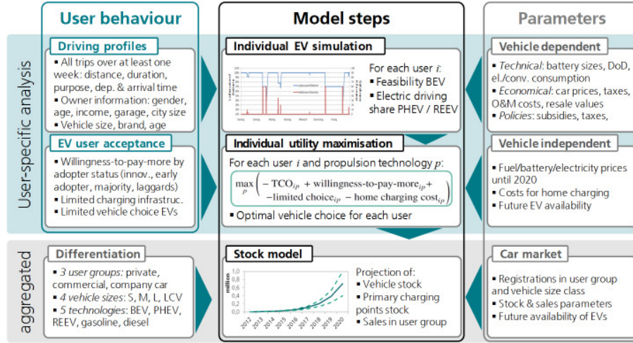
Figure 2: Overview of the proposed model for the market diffusion of electric vehicles using real-world driving data. Based on individual driving data from private, commercial and company cars (left panel) and using techno-economical parameters (right panel), the market shares of different propulsion technologies are determined in three steps (central panel): (1) each driving profile is simulated as EV and conventional vehicle; (2) based on the TCO, the cost for home charging, the limited choice of EV makes and models and the individual willingness-to-pay-more the utility maximising vehicle option is chosen for each driving profile; (3) the vehicle choices are extrapolated to market shares and aggregated to a vehicle stock.
