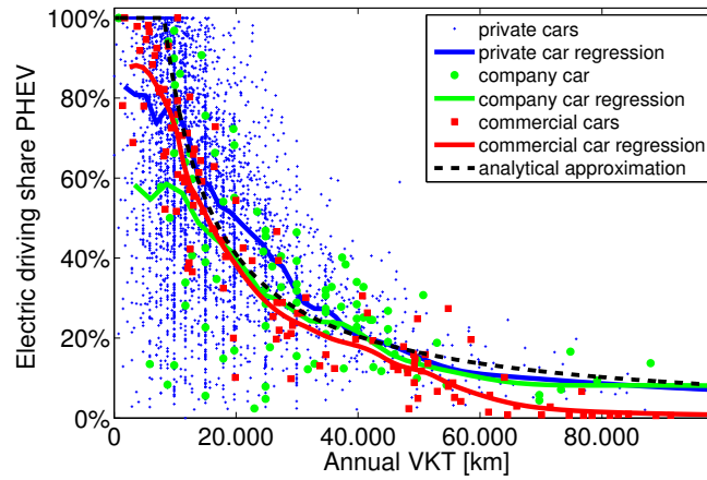
Figure 4: Simulated PHEV electric driving shares as a function of annual VKT for medium-sized vehicles. Shown are the results of battery simulations of many individual cars (symbols) and a kernel regression (solid lines): private (blue, N = 3561 ), company cars (green, N = 117 ) and commercial cars (red, N = 96 ). A simple approximation for the kernel regression given by s(r) = 240 \cdot L/r (dashed black line) is also shown.
