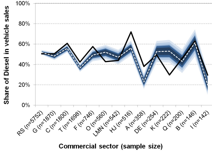
Figure 3: Diesel market shares within different branches of industry in Germany. Shown are the actual values from a large-scale survey (solid line) and the estimate from a simple TCO calculation (dashed line) together with confidence bands (in blue - see section 4.2) from the finite sample sizes (given in parentheses). See text for details of the calculation.
